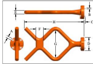
"F" Handle
