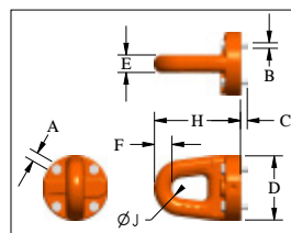
"Eye" Handle
