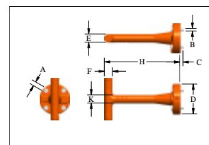
"T" Handle
