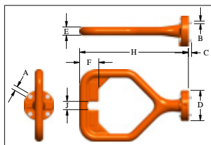
"D" Handle
