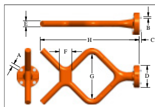
"F" Handle
