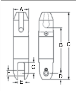
AS-14 Thimble & Bullet
