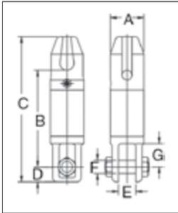
AS-11 Thimble & Jaw
