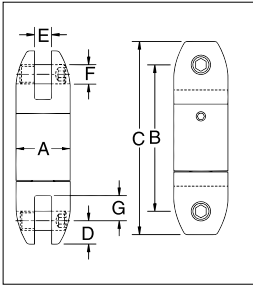
AS-7 Bullet Style Jaw & Jaw
