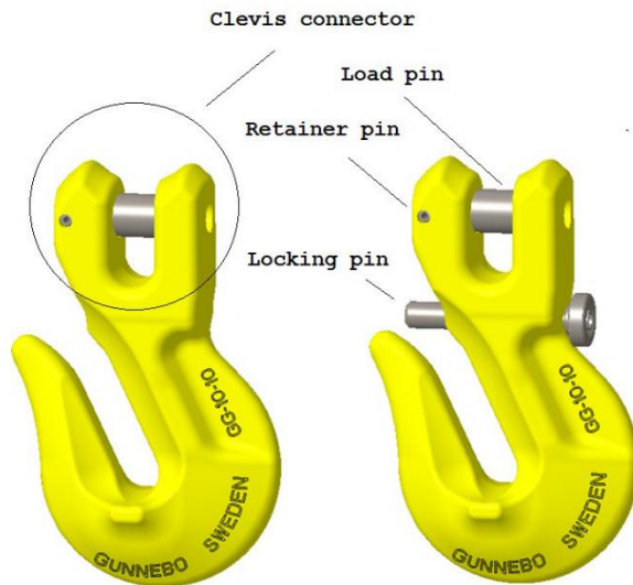
Figure 7: Grab Hook GG Grade 10 and Grab Hook GG LP Grade 10
